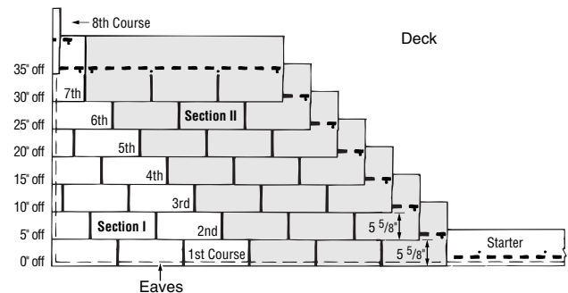
Figure 10-15: Eight-Course, Five-Inch, Stepped-Off Diagonal Method.
